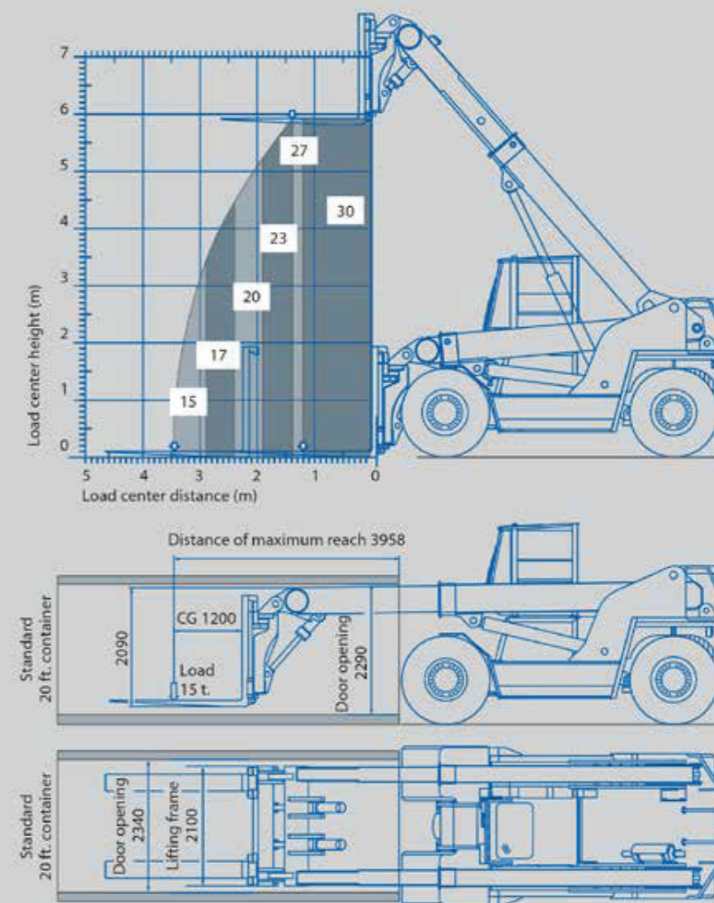
Lifting capacity diagram and working dimensions ML3012RC
